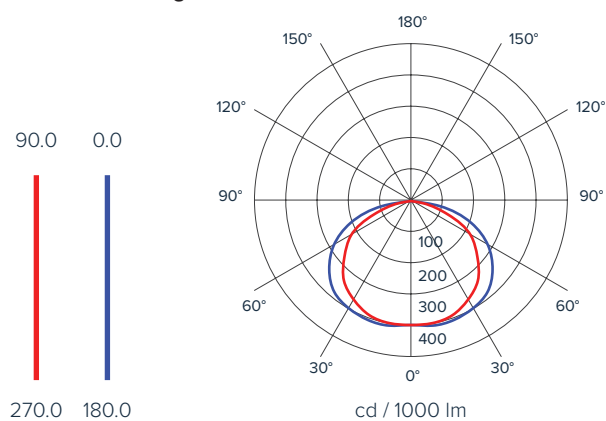
Photometric diagram
