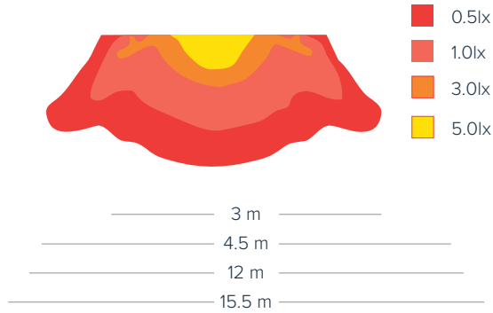
Symmetrical lens
