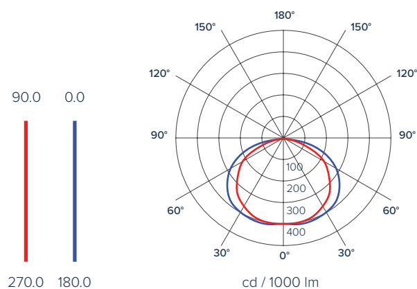
18W and 24W photometric diagram
